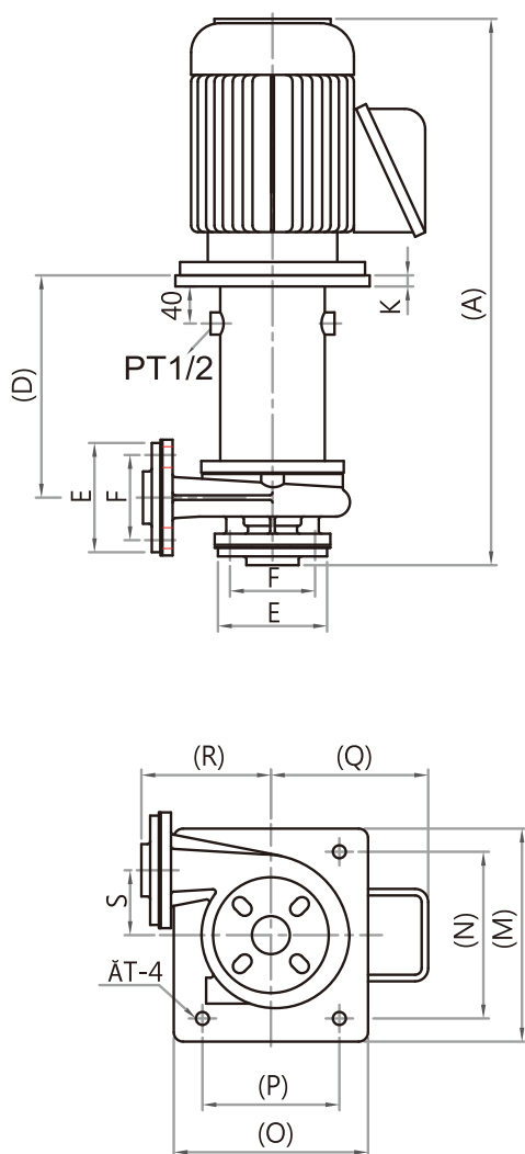
DIMENSION 尺寸表 SV-IN/OUT-Female screw (內牙式)/JIS 5K
